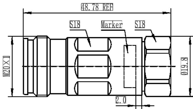
43F-SCF12-C03 Outline Drawing
